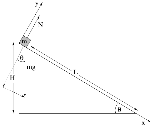
Figure 11: A good choice of coordinate frame has (say) the x -coordinate lined up with the total force and hence direction of motion.
