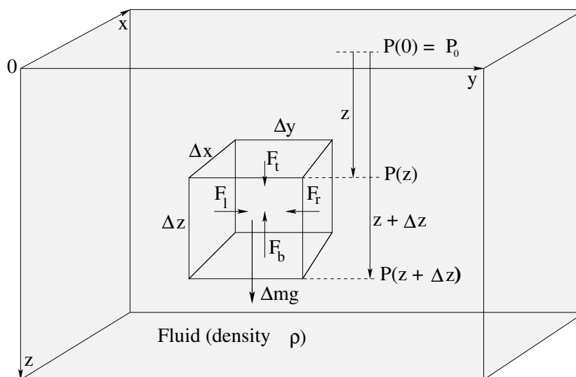
Figure 103: A fluid in static equilibrium confined to a sealed rectilinear box in a near-Earth gravitational field \vec{g} . Note well the small chunk of fluid with dimensions \Delta x, \Delta y, \Delta z in the middle of the fluid. Also note that the coordinate system selected has z increasing from the top of the box down , so that z can be thought of as the depth of the fluid.
