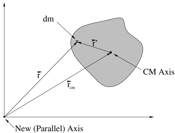
Figure 76: An arbitrary blob of total mass M rotates around the axis at the origin as shown. Note well the geometry of \vec{r}_{cm} , \vec{r}' , and \vec{r} = \vec{r}_{cm} + \vec{r}' .
