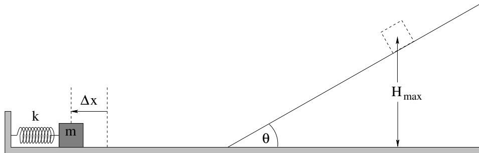
Figure 41: A spring compressed an initial distance \Delta x fires a mass m across a smooth ( \mu_k \approx 0 ) floor to rise up a rough \mu_k \neq 0 ) incline. How far up the incline does it travel before coming to rest?
