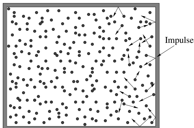
Figure 101: A large number of atoms or molecules are confined within in a “box”, where they bounce around off of each other and the walls. They exert a force on the walls equal and opposite the force the walls exert on them as the collisions more or less elastically reverse the particles’ momenta perpendicular to the walls.
