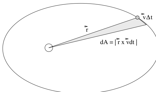
Figure 154: The area swept out in an elliptical orbit in time \Delta t is shaded in the ellipse above.
