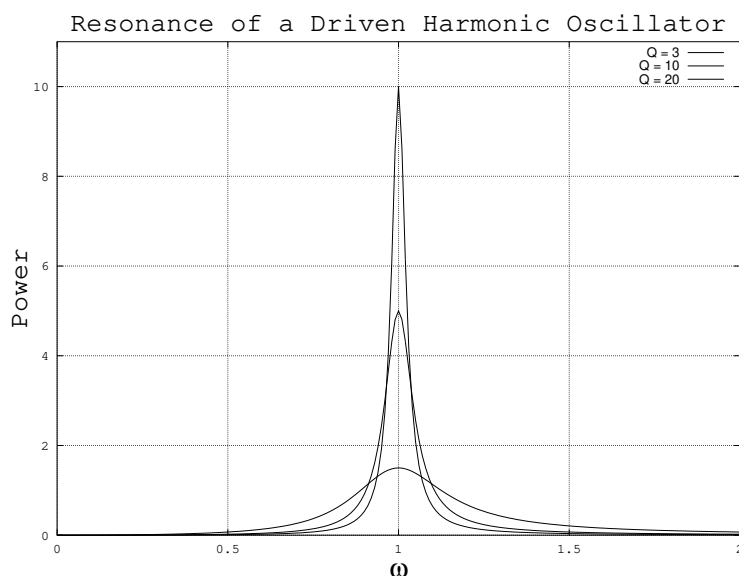
Figure 130: This plots the average power P(\omega) for three resonances. In these figures, F_0 = 1 , k = 1 , m = 1 (so \omega_0 = 1 ) and hence b is the only variable. Since Q = \omega_0/\Delta = m\omega_0/b we plot Q = 3, 10, 20 by selecting b = 0.333, 0.1, 0.05 . Thus P_{\max} = F_0^2/2b = 3/2, 5, 10 respectively (all in suitable units for the quantities involved). Note that the full width of e.g. the Q = 20 curve (with the sharpest/highest peak) is \sim 1/20 at P = P_{\max}/2 = 5 . P is the average power added to the oscillator by the driving force, which in turn in steady state motion must equal the average power lost to dissipative drag forces.
