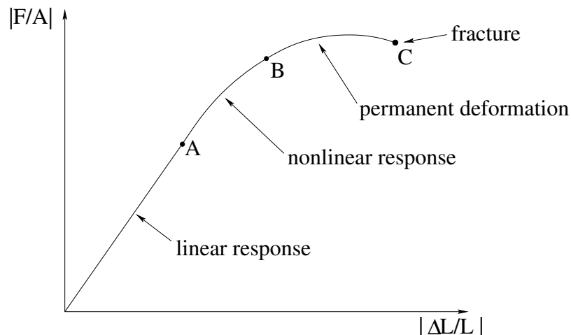
Figure 134: The slope of the linear response part of the curve is Young’s Modulus (note well the absolute magnitude signs). A marks the point where nonlinear response is first apparent. B marks the boundary where dislocations occur and permanent deformation of the material begins. C marks the point where there is a chain reaction – each defect produced produces on average at least one more defect at the same stress, so that the material “instantly” fractures.
